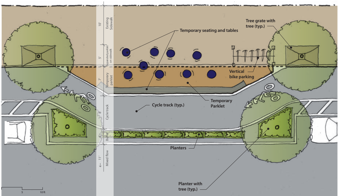
Figure 19: Cycle Track with Parklet Integration
