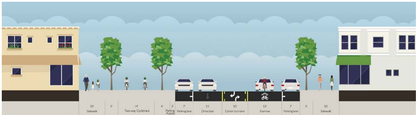
C1 - 4 LANE with CYCLETRACK (TWO-WAY)
